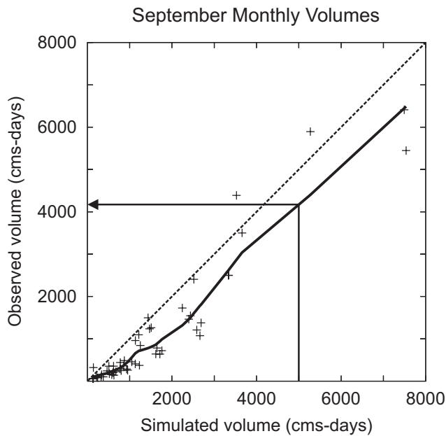
Fig. 3. Illustration of the LOWESS regression method. The crosses show observed and simulated monthly flow volumes from the historical simulation. The solid line shows the LOWESS regression. The arrow illustrates the transformation of an ensemble trace to the bias-corrected ensemble trace.
