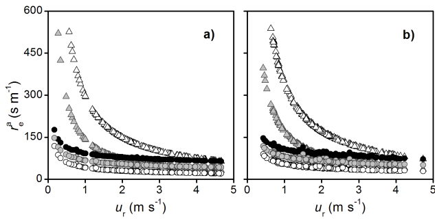
Fig. 4. Effective aerodynamic resistances ( r_a^e ) plotted against the wind speed at reference height ( u_r ): r_{a_1}^e ( \Delta ), r_{a_2}^e ( \Delta ), \langle r_{a_p}^e \rangle ( \circ ), \langle r_{a_s}^e \rangle ( \bullet ) and \langle r_a^e \rangle ( \circ ). (a) R. sphaerocarpa patch; (b) Herbaceous patch.
