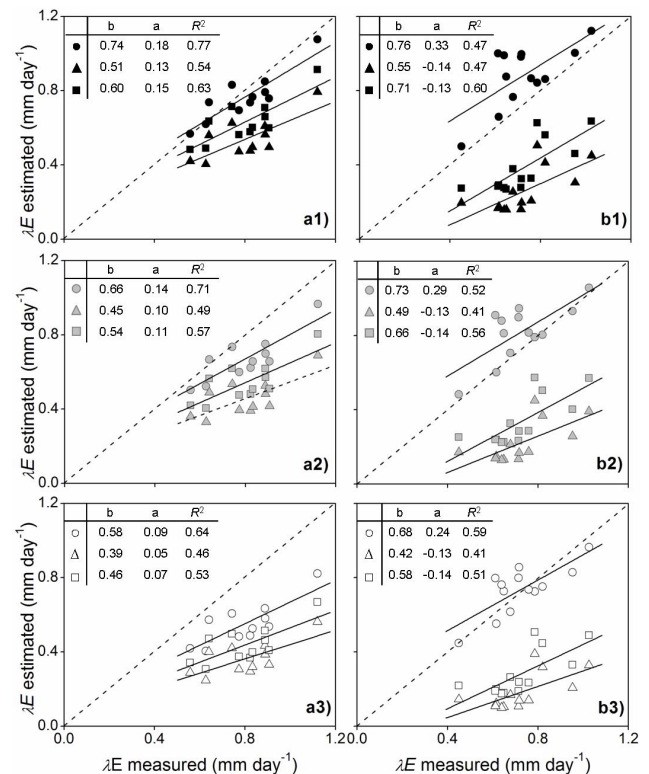
Fig. 9. Regressions between estimated and measured \lambda E for the R. sphaerocarpa patch (panels a1, a2, and a3) and the herbaceous patch (panels b1, b2, and b3). \lambda E was estimated using different combinations of effective surface and aerodynamic resistances: \langle r_s^e \rangle_p and \langle r_a^e \rangle_s (●); \langle r_s^e \rangle_p and \langle r_a^e \rangle_p (○); \langle r_s^e \rangle_s and \langle r_a^e \rangle_s (■); \langle r_s^e \rangle_s and \langle r_a^e \rangle_p (□); \langle r_s^e \rangle_s and \langle r_a^e \rangle_s (▲); \langle r_s^e \rangle_s and \langle r_a^e \rangle_p (Δ). The regression lines (solid lines) and 1:1 line (dashed line) are shown, as well as the values of slope (b), intercept (a) and R^2 for each of the regressions.
