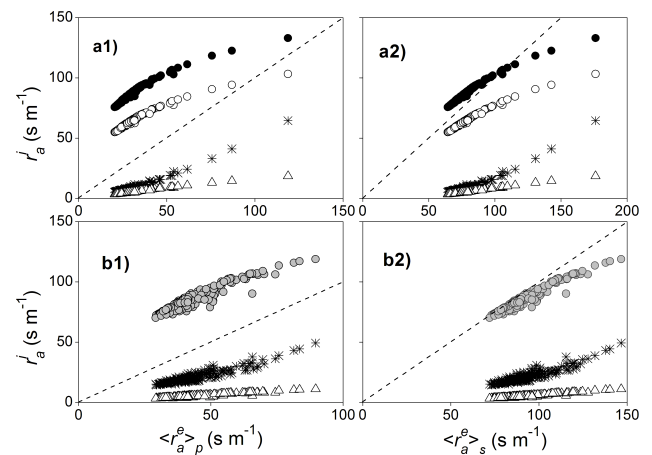
Fig. 6. Aerodynamic resistances of the sources ( r_a^{su} : \bullet ; r_a^{bs} : \circ ; r_a^s : \bullet ; r_a^p : \Delta ) and r_a^a ( \times ) plotted against the effective aggregated aerodynamic resistances: \langle r_{a_p}^e \rangle (a1 and b1) and \langle r_{a_s}^e \rangle (a2 and b2). Plots (a1) and (a2) are for the R. sphaerocarpa patch, and plots (b1) and (b2) are for the herbaceous patch. The dashed line is the 1:1 line.
