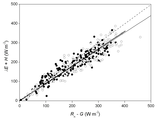
Fig. 3. Comparison of turbulent fluxes ( \lambda E + H ) and measured available energy ( R_n - G ) in the two patches studied: \circ R. sphaerocarpa patch ( n=177 ); \bullet herbaceous patch ( n=197 ). The regression lines forced through the origin are shown (thin line: R. sphaerocarpa patch; thick line: herbaceous patch), and the 1:1 line (dashed line).
