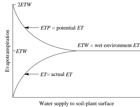
Figure 1. A schematic representation of the complementary relationship between ET, ETW and ETP (after Morton, 1983).
