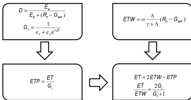
Figure 7. Schematic showing the structure of the proposed GG18 model.
