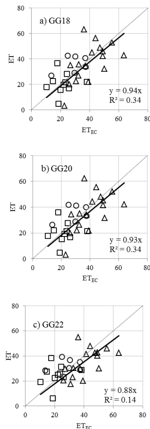
Figure 5. Scatter plots of average ET estimates (mm month -1 ) for GG18, GG20 and GG22 model variations in comparison to measured ET_{EC} fluxes from 33 sites (all except site 4) in the wet (triangle), moderate (circle) and dry (square) climatic classes.
