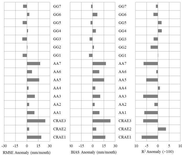
Figure 3. Anomalies of RMSE, BIAS and R^2 values for 17 model variations across the 34 sites. Here anomalies are computed based on the values computed with each corresponding complementary method.
