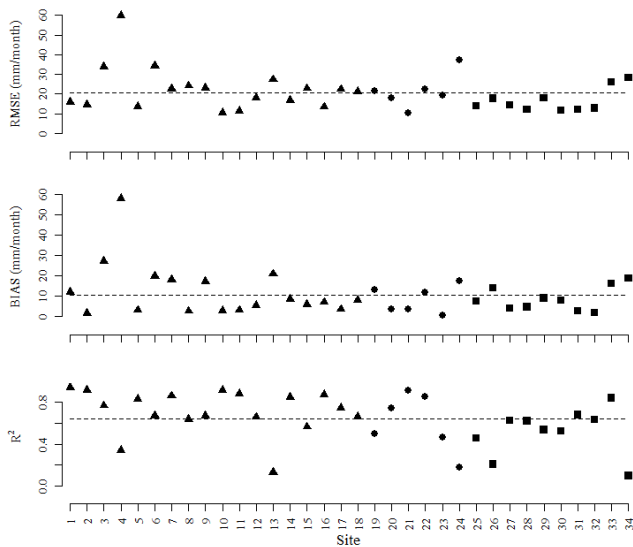
Figure 6. RMSE, BIAS and R^2 of the GG18 model variation at each site in the wet (triangle), moderate (circle) and dry (square) climatic classes and the dashed lines indicate the average values.
