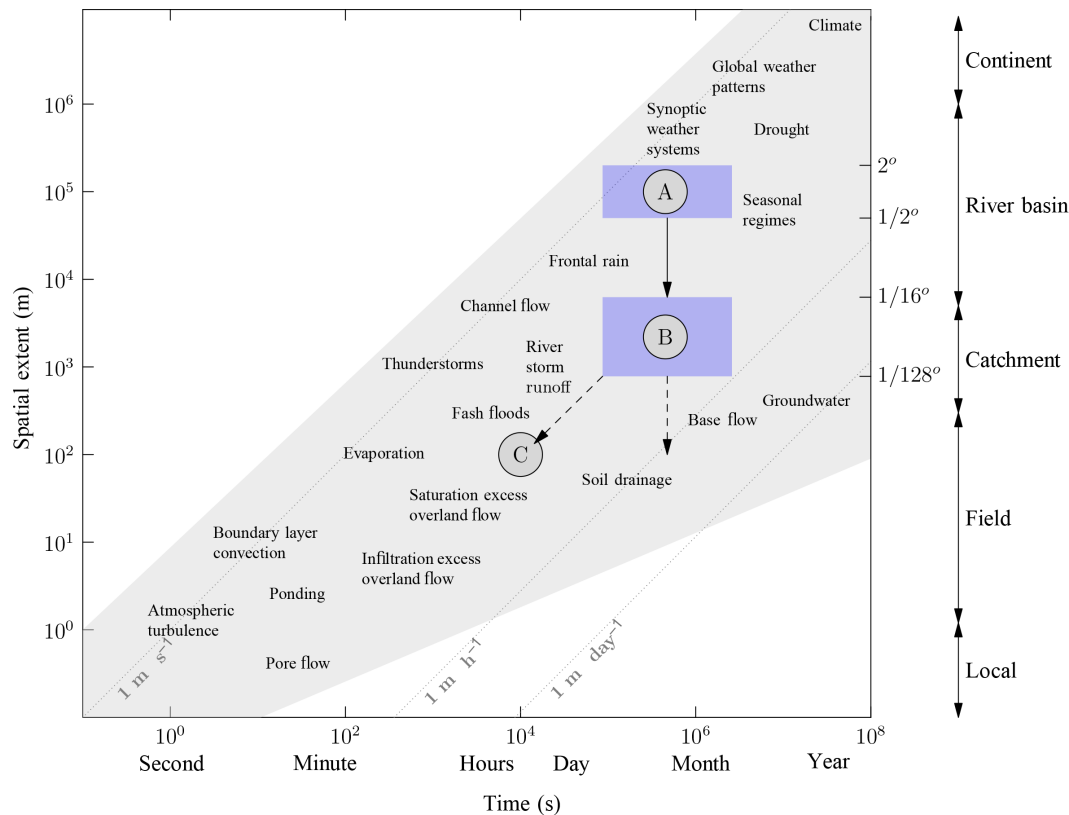
Figure 1. The timescales and space scales of several hydrometeorological processes. Adapted from Brutsaert (2005) and Blöschl and Sivalapan (1995), who based it on Orlanski (1975), Dunne (1978), Fortak (1982), and Anderson and Burt (1990). The blue areas indicate the temporal and spatial resolution at which the VIC model has been applied, when it was initially developed (A) and presently (B). The dashed arrow pointing downwards shows the ambitions of spatial hyper-resolution modelling, whereas the dashed arrow pointing towards (C) shows the temporal and spatial resolution of hyper-resolution modelling if it follows the direction of characteristic velocity of hydrometeorological processes.
