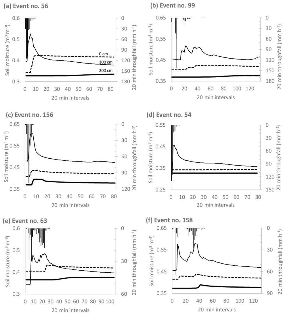
Figure 6. Volumetric soil moisture response at three depths during the six largest events (Table 2). Events with initial surface soil moisture ( 0\text{ cm}) \geq 0.40\text{ m}^3\text{ m}^{-3} are considered to have wet antecedent conditions: 56 (116 mm of rainfall); 99 (111 mm); 156 (89 mm); and 158 (78 mm). The other two events, 54 (81 mm) and 63 (77 mm), are associated with drier antecedent moisture conditions ( \leq 0.30\text{ m}^3\text{ m}^{-3} ). All data are plotted as 20 min aggregated values. Soil moisture curves in all panels correspond to surface (thin line), 1 m (dashed line), and 2 m (thick line) depths (key shown in panel a). Each rainfall bar represents a 20 min period.
