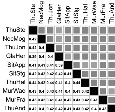
Brown-Resnick m-s
