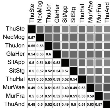
Brown-Resnick m-s
