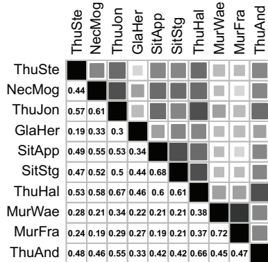
Fisher copula
