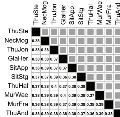
Gaussian m-s
