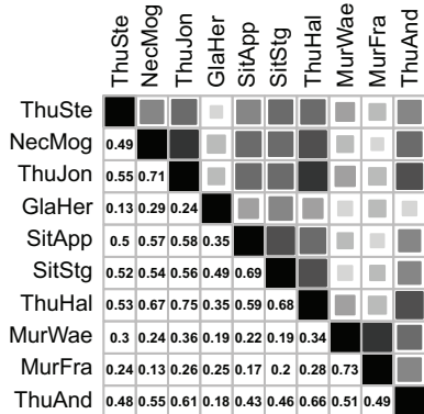
Fisher copula
