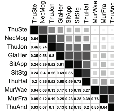
Gaussian m-s
