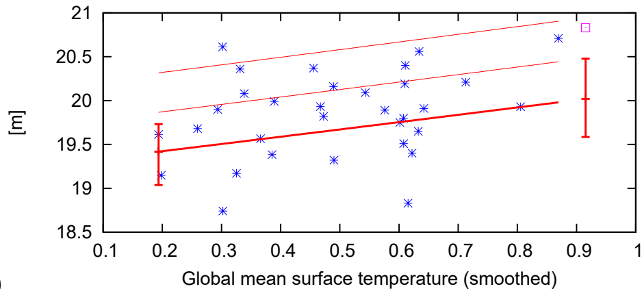
Jul–Sep index water level Bahadurabad 1985:2016 (95 % CI)
