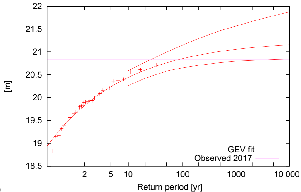
Jul–Sep index water level Bahadurabad 1985:2016 (95 % CI)
